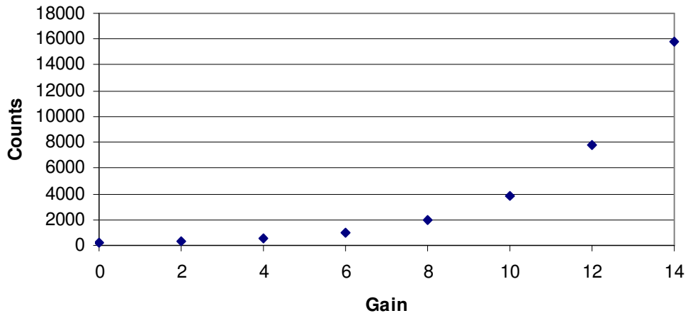
Peak Counts as a function of Gain (Channel 1)
