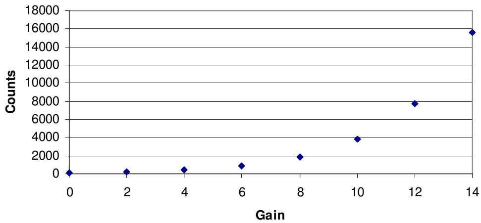
Peak Counts as a function of Gain (Channel 2)
