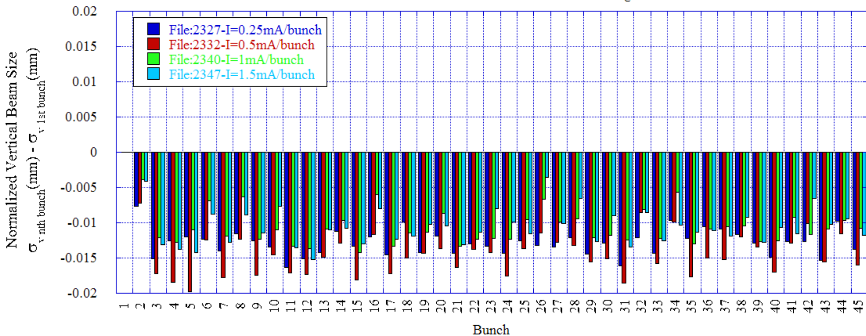
e- Vertical Beam Size for 45 Bunch Train-100 Turn Average
