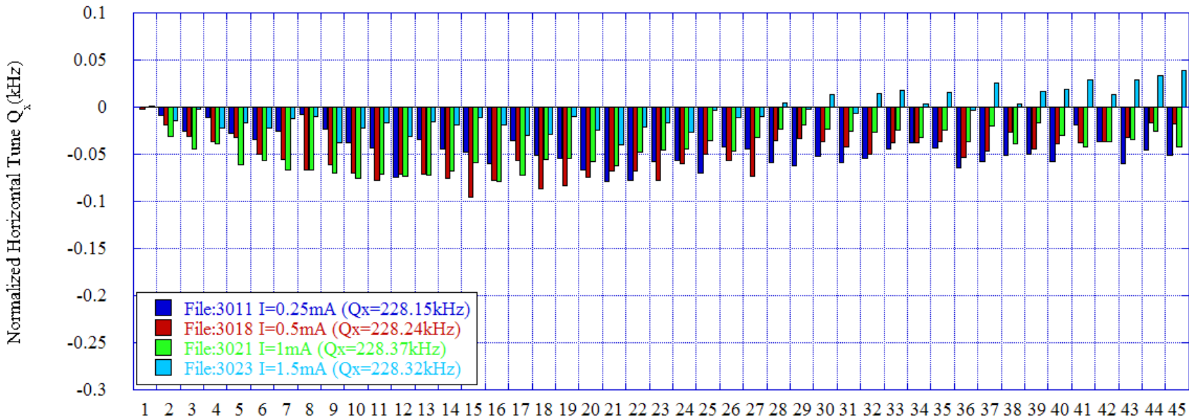
e- Horizontal Tune for 45 Bunch Train
