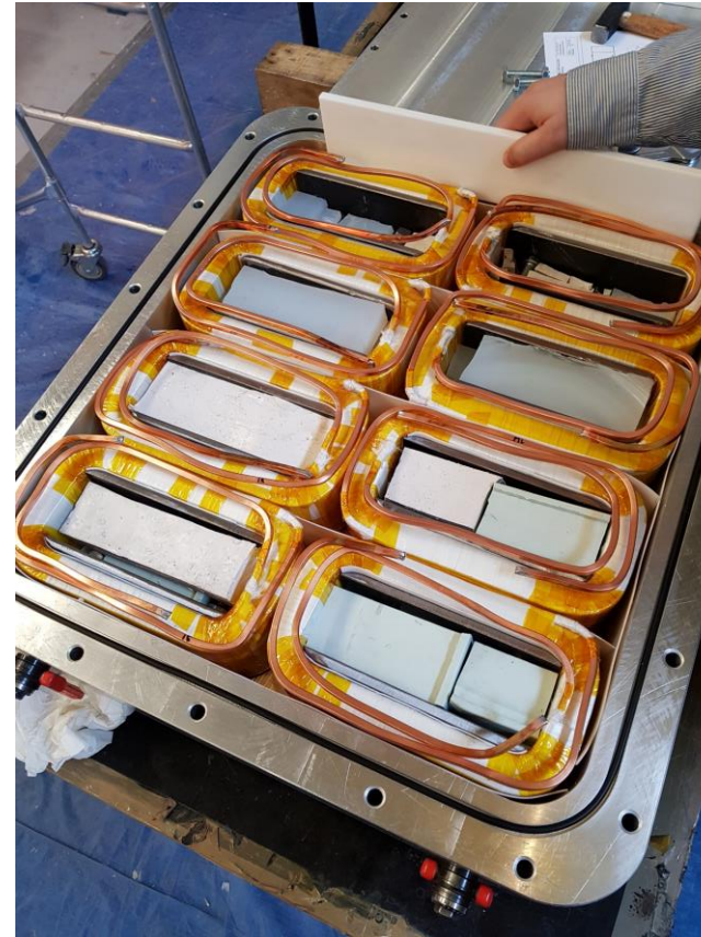
8 DIPOLE COILS: STATUS Impregnation done.
