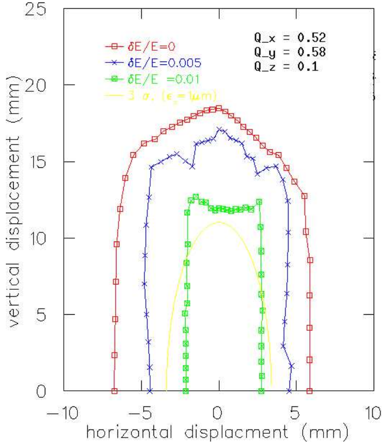
Figure 2: CesrTF dynamic aperture for 0.5% and 1% energy offsets. The smooth yellow curve corresponds to 3\sigma of the the rms size of the injected beam.
