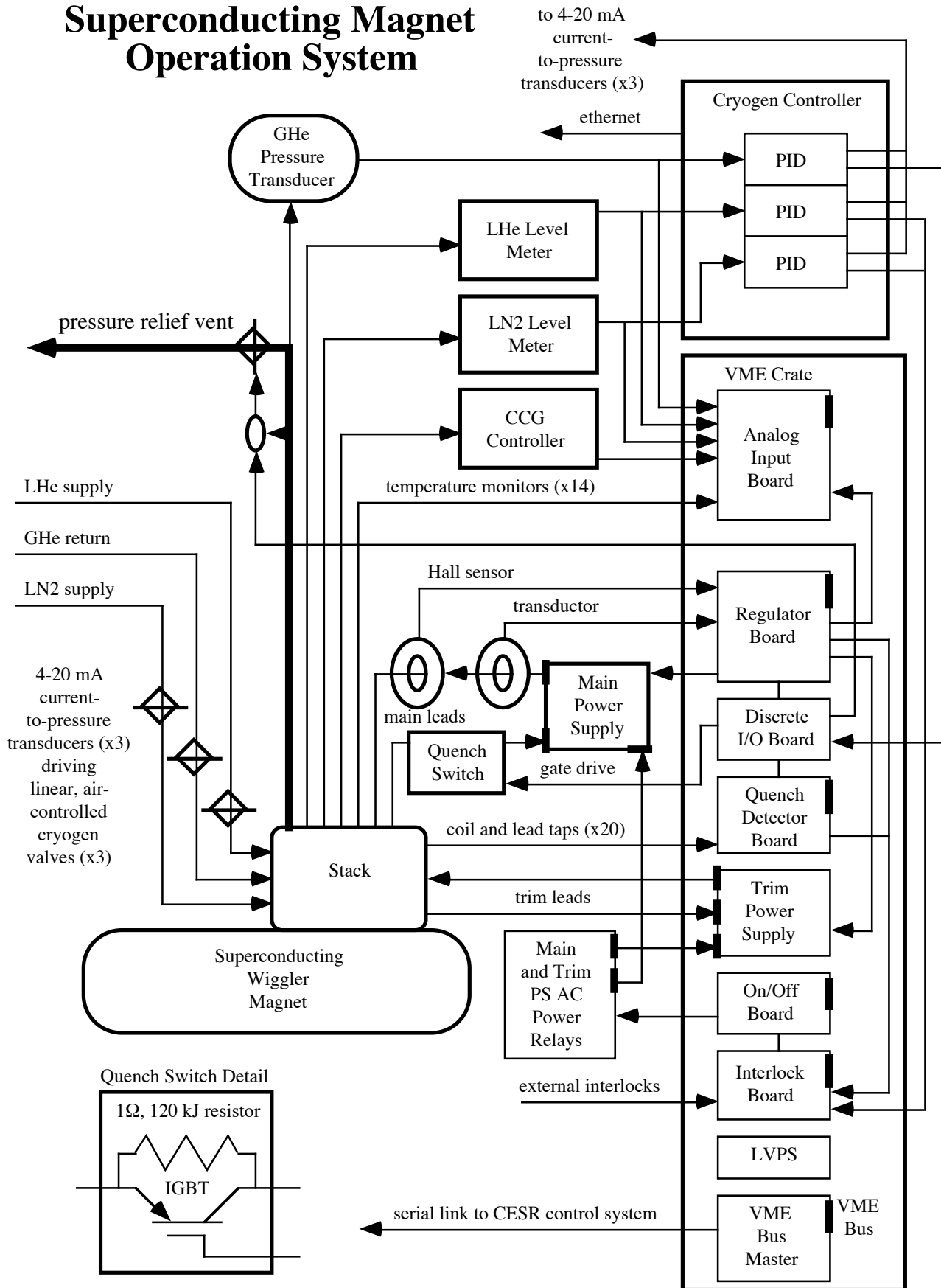
Figure 1: CESR Wiggler Superconducting Magnet Operation System Block Diagram
