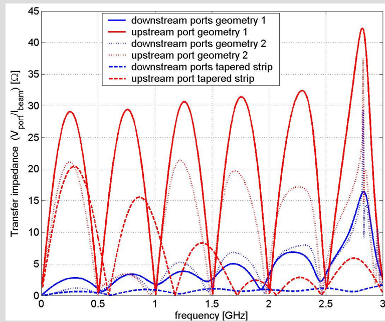
transfer impedance
