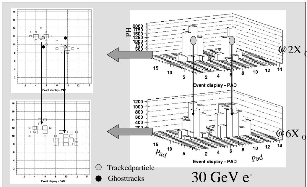
Figure 4: Example of particle separation on the silicon pads. The dots correspond to particle impact prediction using the external telescope. The physical particles are clearly recognised.
